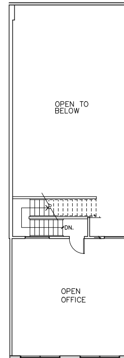
2ND FLOOR
