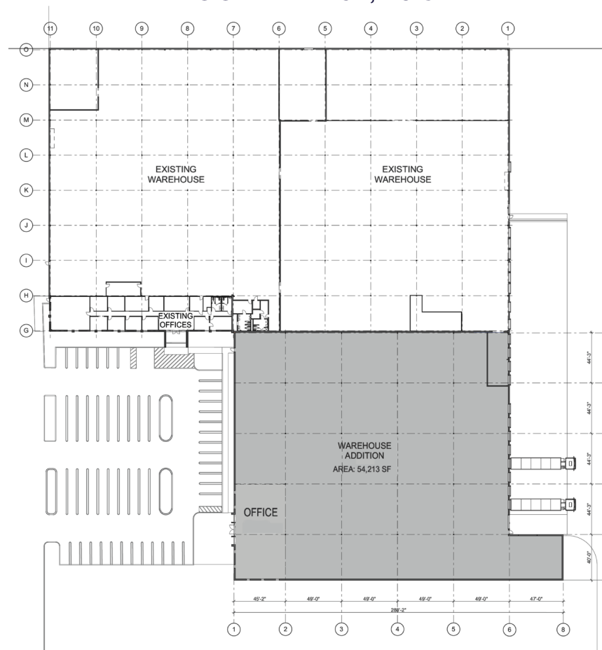
FLOOR PLAN 54,213 SF
