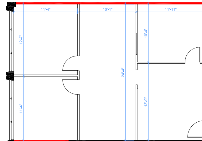
SUITE 205: 970 SF
