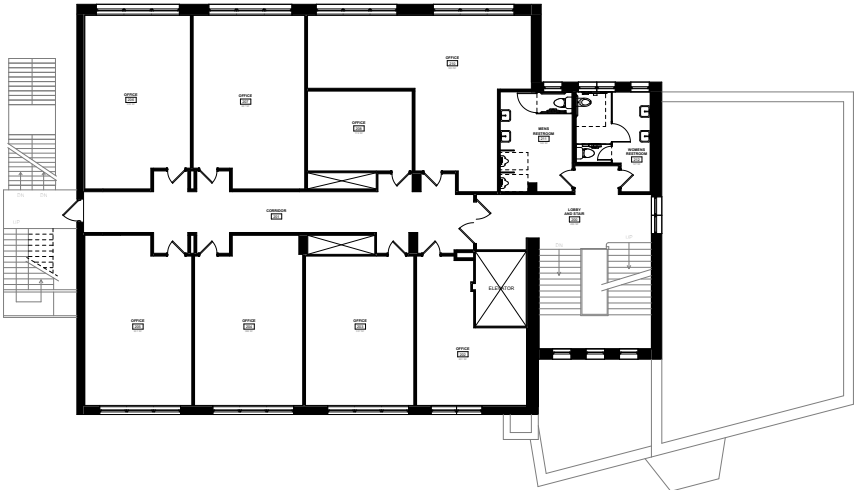
② SECOND FLOOR PLAN
