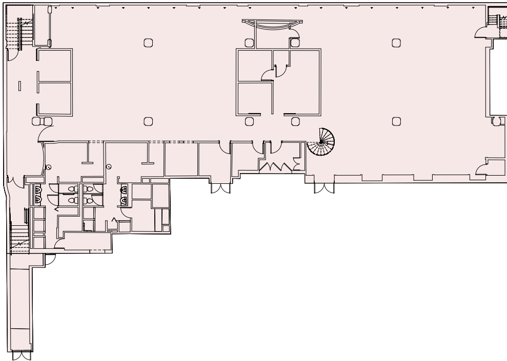
GROUND FLOOR 7,810 SF
