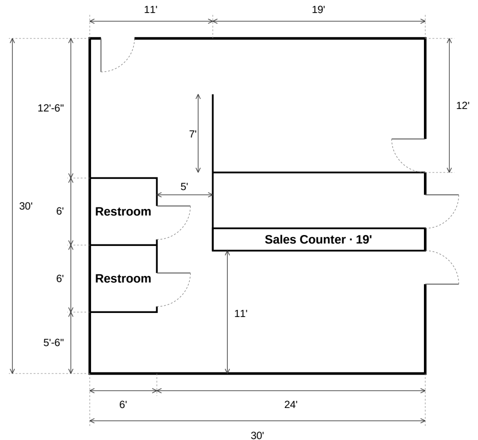
OFFICE FLOOR PLAN
