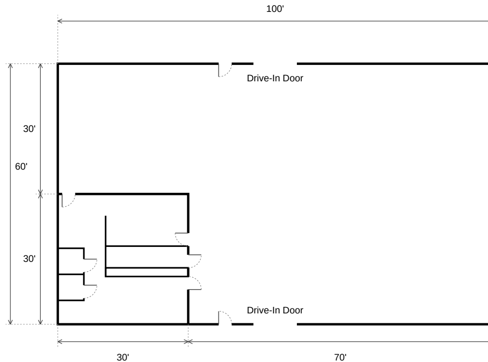
BUILDING FLOOR PLAN
